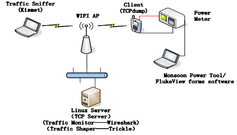
Fig. 4. Experimental setup.
