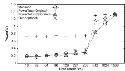
Fig. 10. Power consumption of TCP download with single flow on Nexus S.
