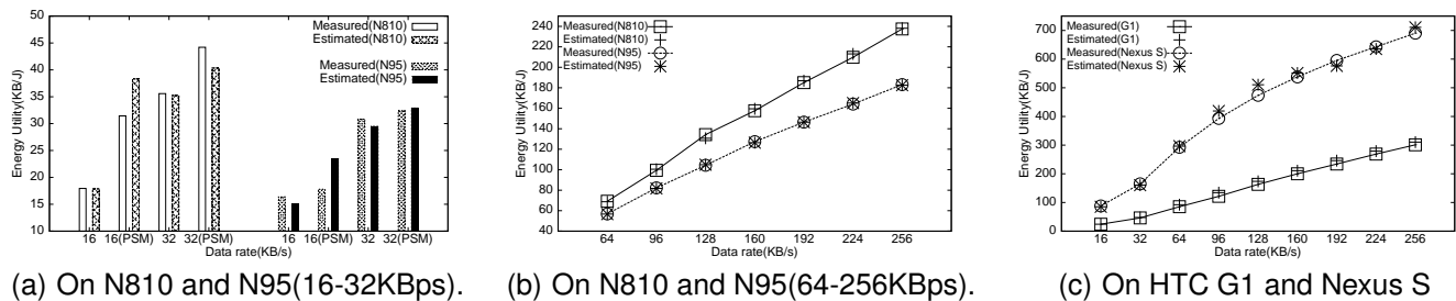
Fig. 5. Energy utility of TCP download with single flow at rate between 16KBps and 256KBps.
